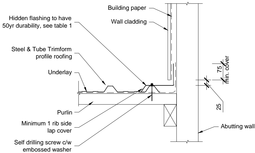
LOW / MEDIUM / HIGH WIND ZONES WHERE PITCH ≥ 10°
