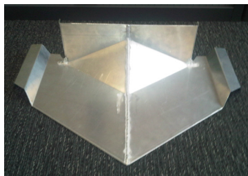
WELDED CRICKET FLASHINGS
