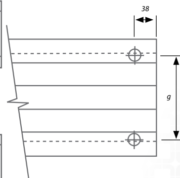
HST 200, HST 250, HST 300, HST 350, HST 400
