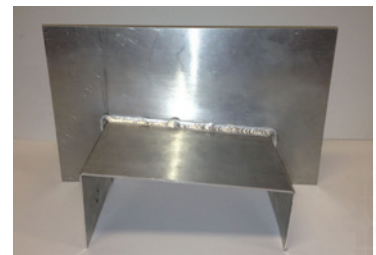
SADDLES
