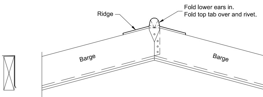
END VIEW
