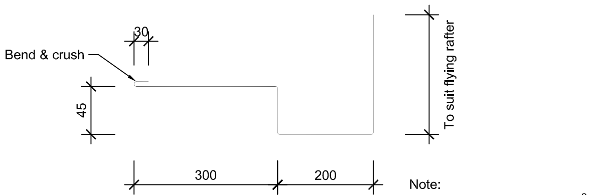
BARGE GUTTER DETAIL SCALE: 1:5
