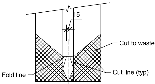
DETAIL RIDGE END CUT
