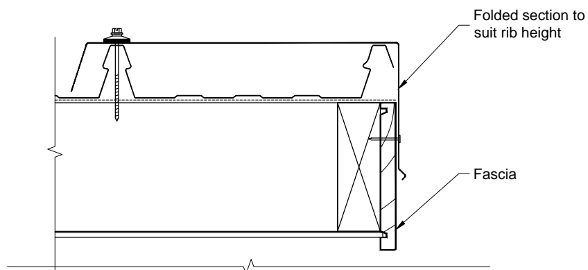
Section AA 1:5
