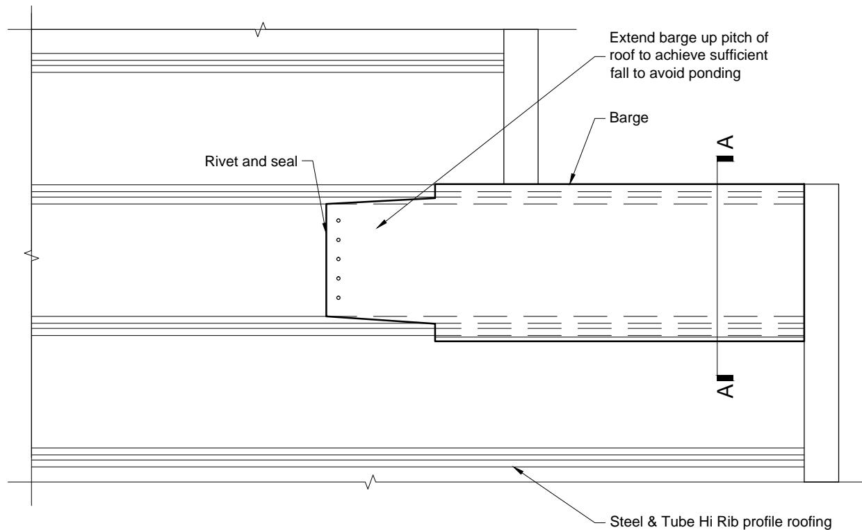
Section AA 1:10
